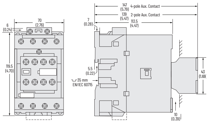
Figure 63 - 100-E40...100-E52 4-Pole Contactors with Front-mounted Auxiliary Contact
